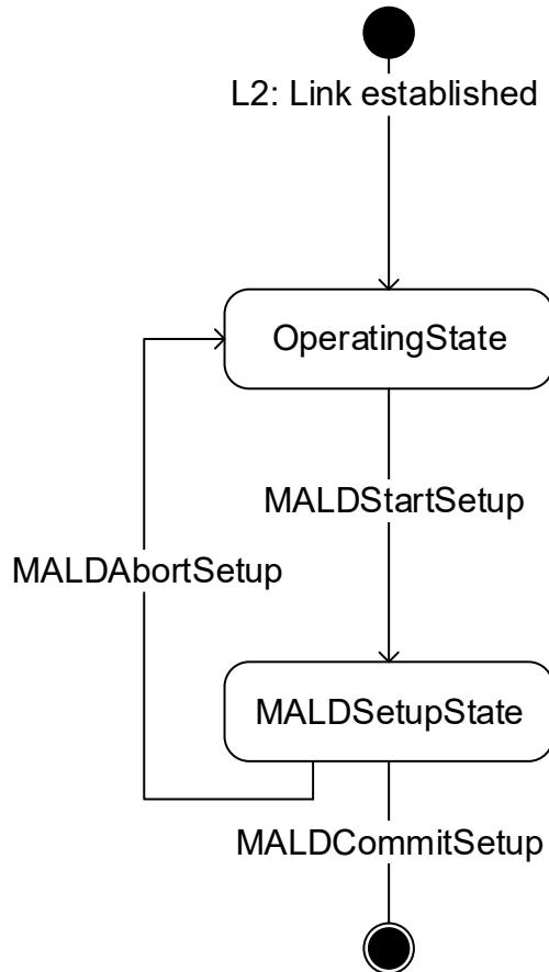
Figure 8.6.3.4-1: MALDSetupState
