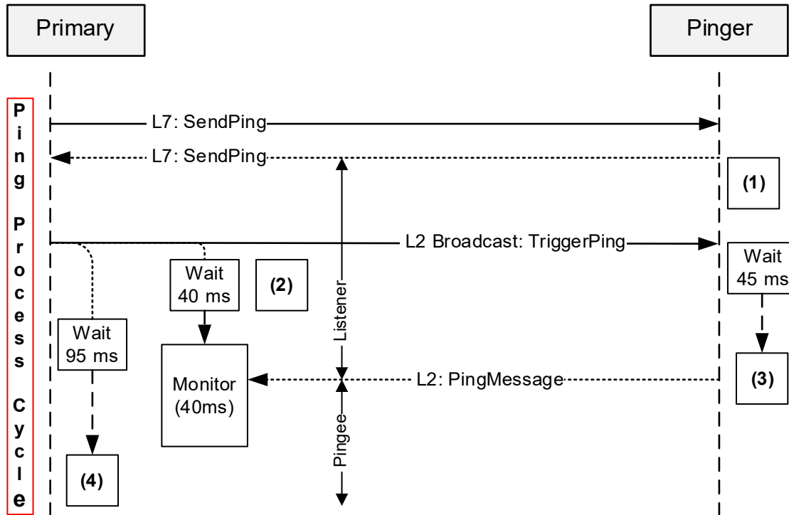
Figure 8.5.5-3: Sequence diagram when the primary receives the Ping message
