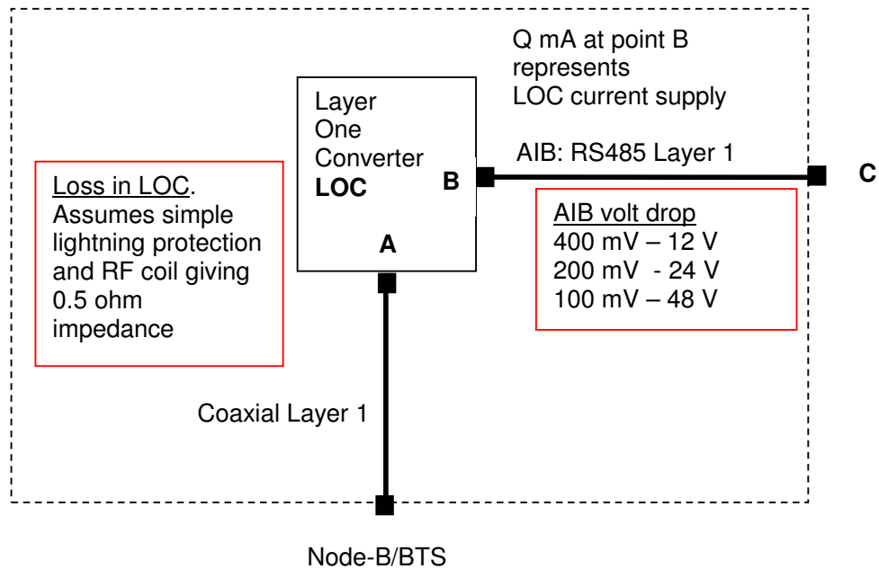
Figure 6.4.4: LOC and RET configuration
