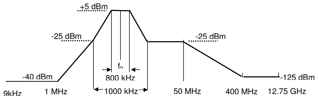
Figure 6.6.6.2: Spectrum mask for modems
